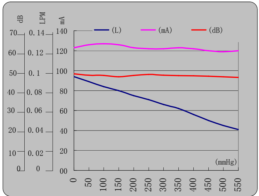
Characteristic Curve:
